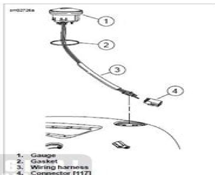
Figure 7-69. Fuel Gauge
