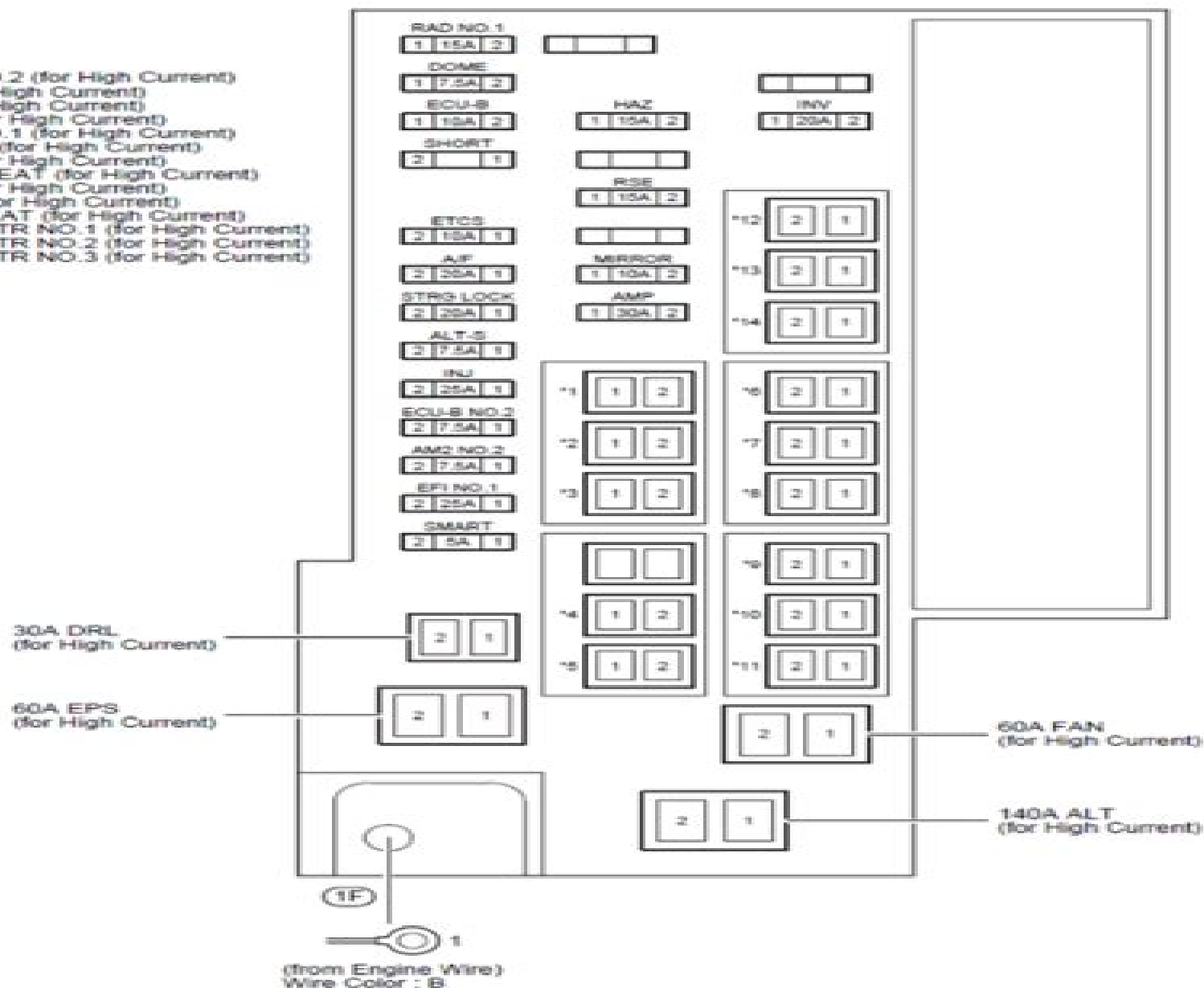
Fig 14: Engine Room J/B Fuse Locations (Top View)
