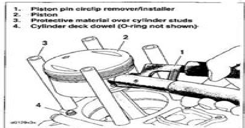
Figure 3-27. Piston Pin Circlip Removal (Part No. HD-42317)
