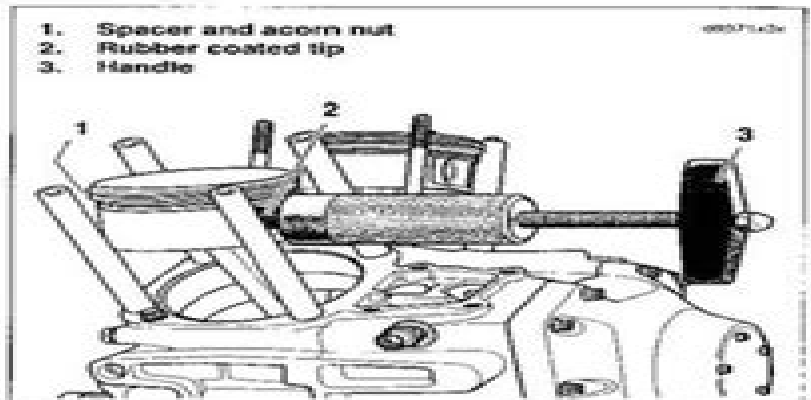
Figure 3-28. Piston Pin Remover (Part No. HD-42320-A)
