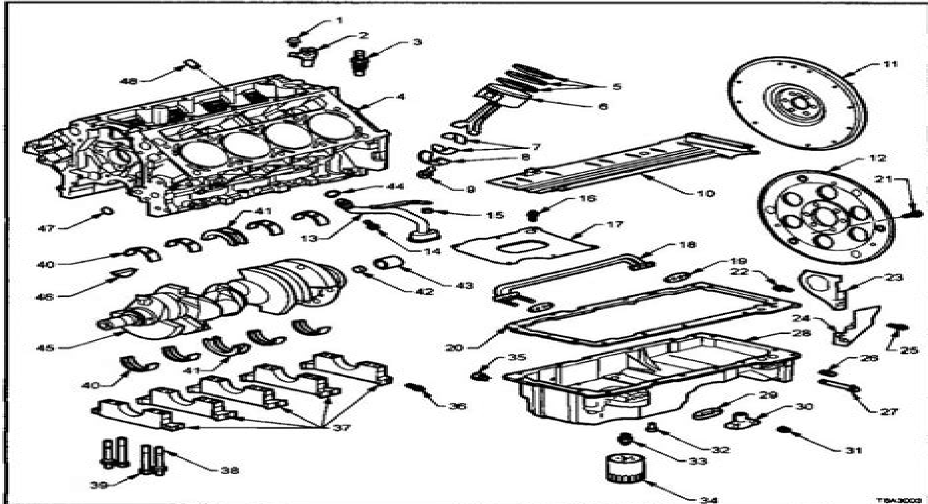
Figure 8A3-3 - Lower Engine Assembly
