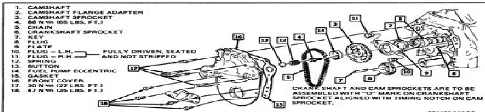
Fig. 32 Front of Engine
