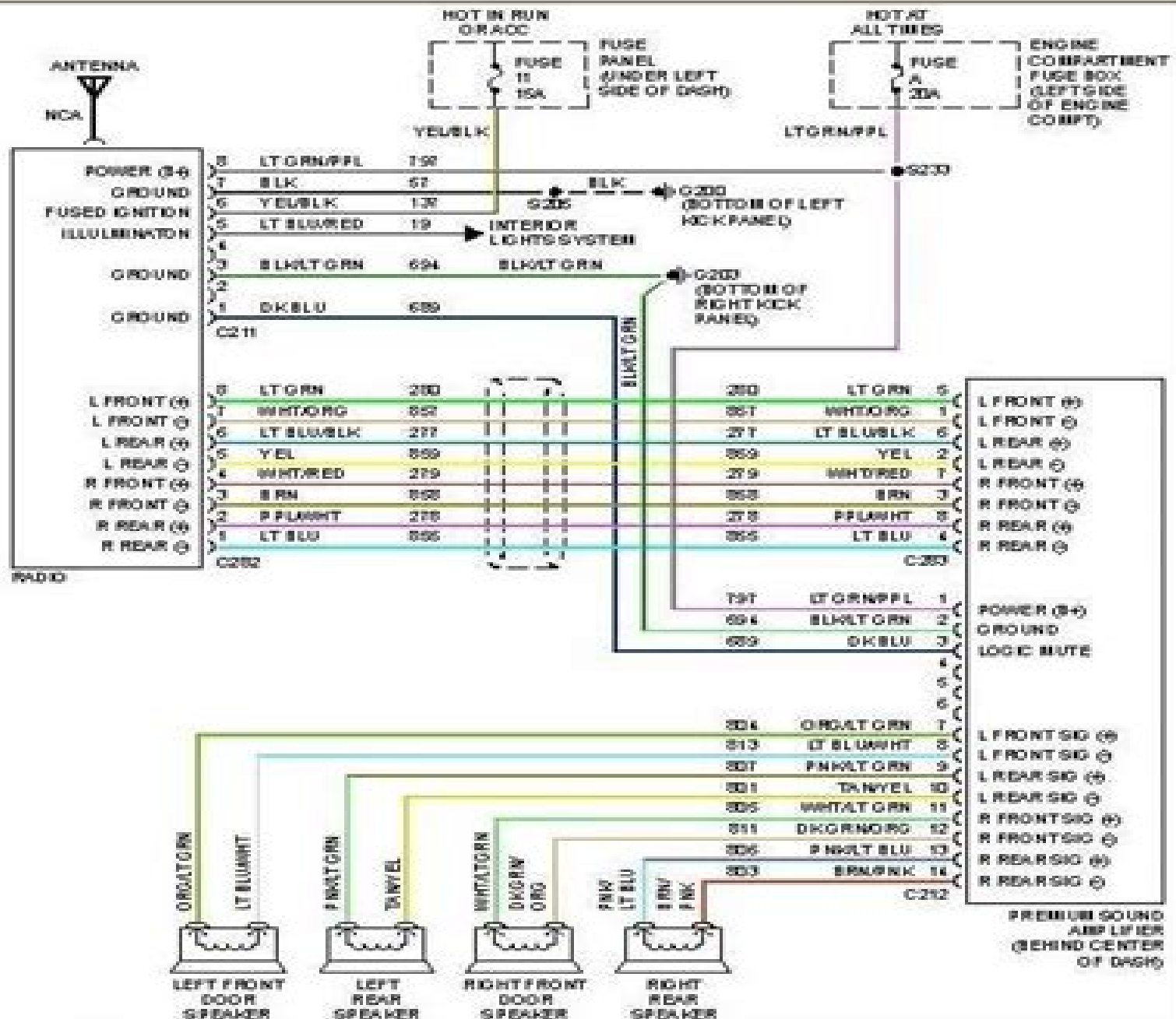
Fig. 58: Premium Sound Radio Circuit
