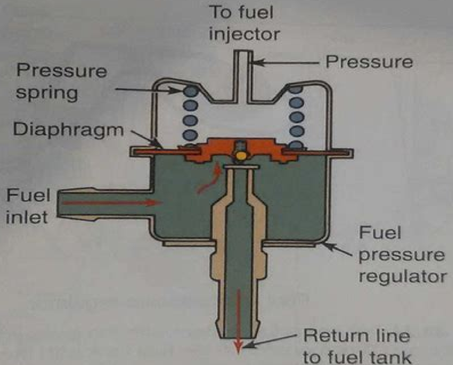
Figure 40.22 A fuel pressure regulator.
