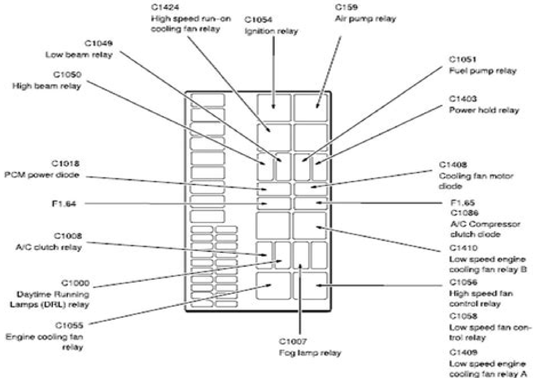
Battery Junction Box (BJB)
