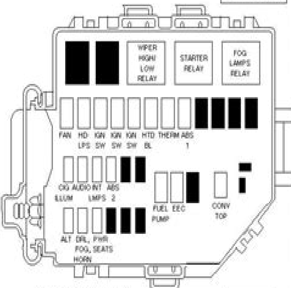
MAXI-FUSE CARTRIDGE TOP VIEW
