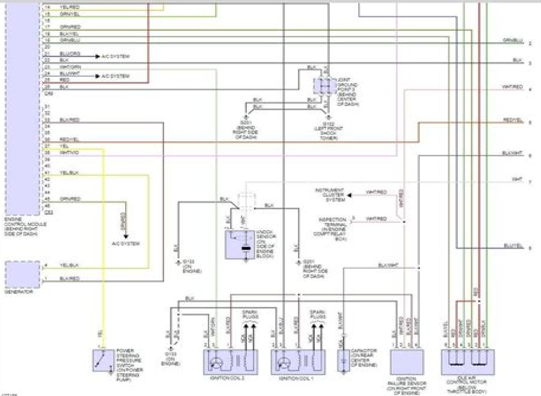
Fig 1: 2.4L Engine Performance Circuits, W/ M/T (1 of 2)
