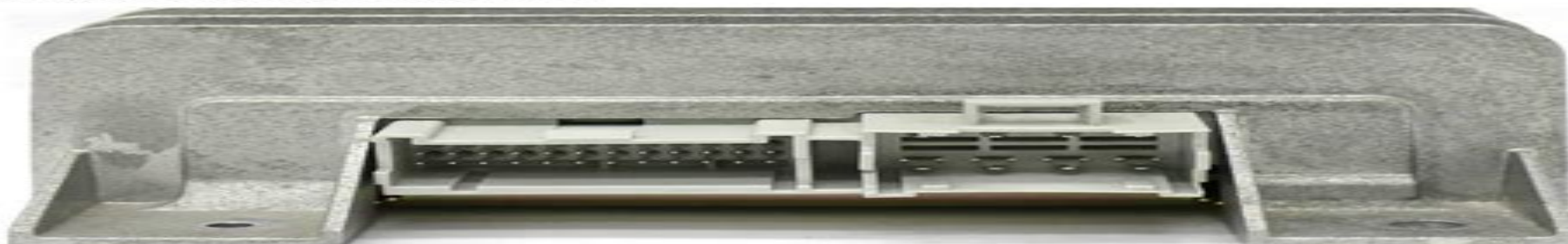
24 pin GMC 12110244, 12110088 (15306210) Radio Harness connector at the car stereo harness (connector end view)
