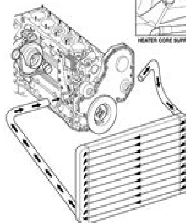
Fig. 2 Cooling System Circulation—Diesel Engine
