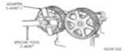
Fig. 42 Crankshaft Sprocket—Removal/Installation
