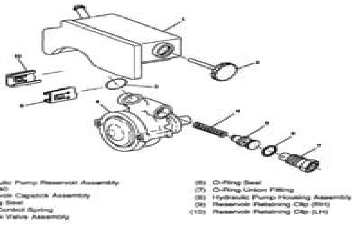
Fig. 5: Exploded View Of Power Steering Pump Assembly-CB Series Courtesy of GENERAL MOTORS CORP.
