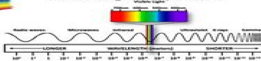
Electromagnetic Spectrum
