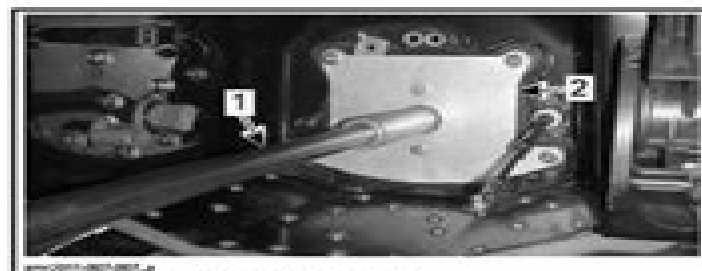
1. Alignment shaft (PN 295 000 141) 2. Alignment tool
