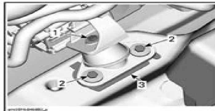
REAR STARBOARD ENGINE MOUNT SHOWN 1. Engine mounting screw 2. Engine mount retaining screws 3. Shim(s)
