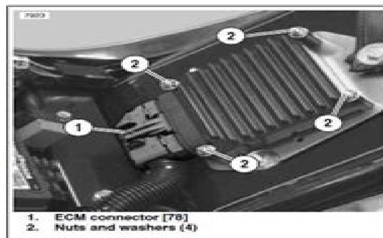
Figure 9-13. ECM Mount: FXSTI/FXSTBI/FXSTS/FXSTDI
