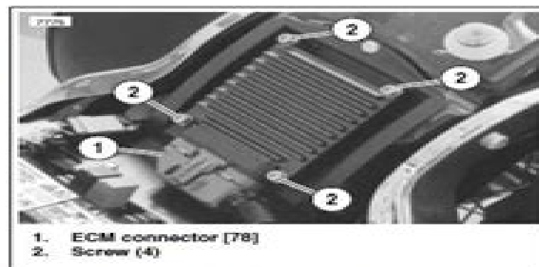
Figure 9-12. ECM Mount: All But FXSTI/FXSTBI/FXSTS/FXSTDI
