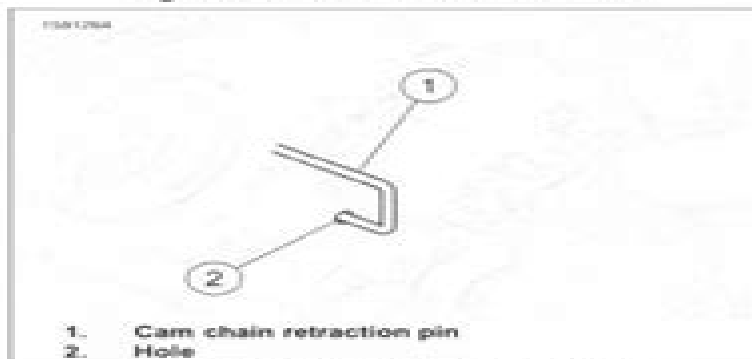
Figure 4-30. Cam Chain Retraction Pin
