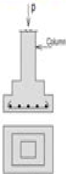
(b) Stepped Footing
