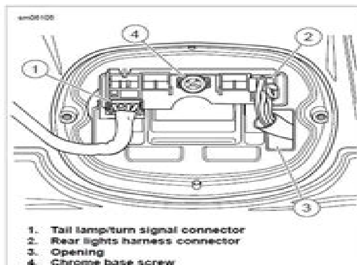
Figure 2-25. Remove Lens From Chrome Base
