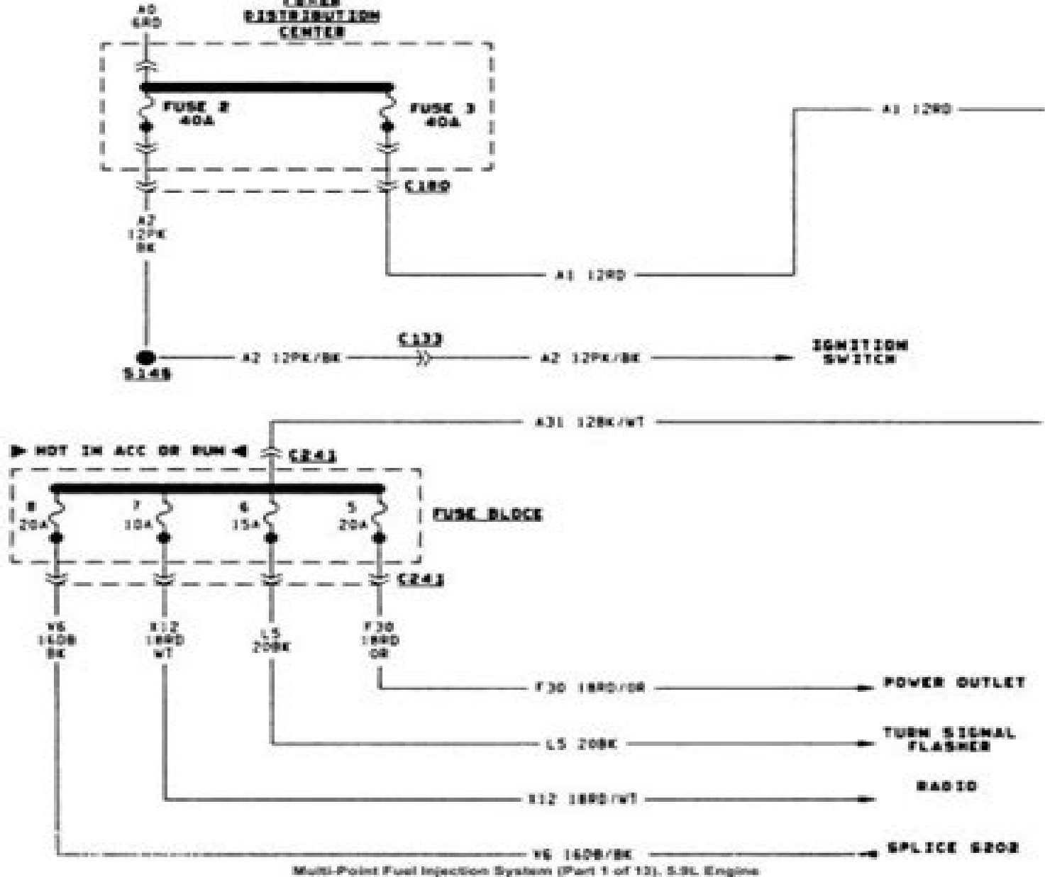
Multi-Point Fuel Injection System (Part 1 of 13), 5.9L Engine
