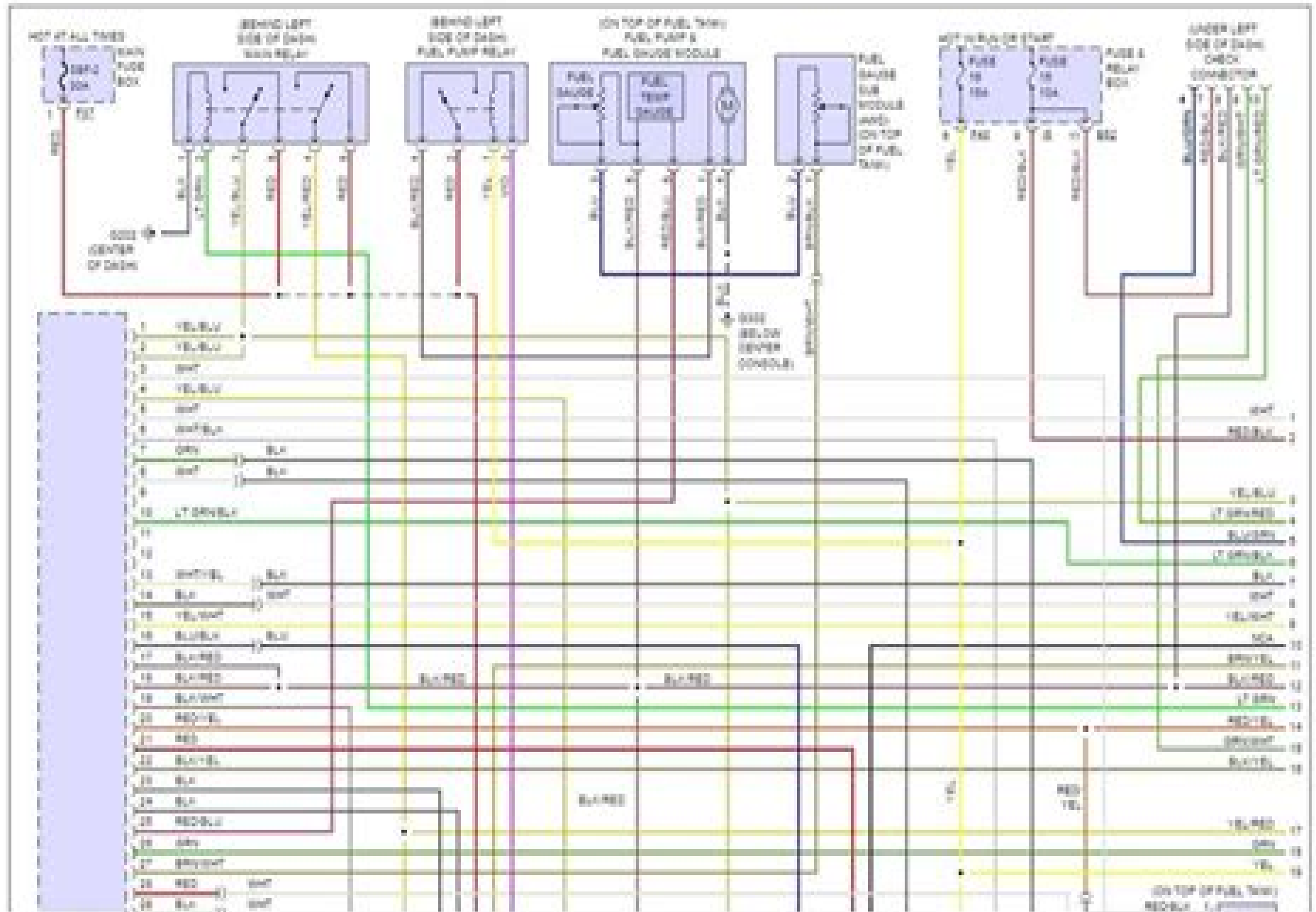
Fig 1: 2.2L Engine Performance Circuits (1 of 2)
