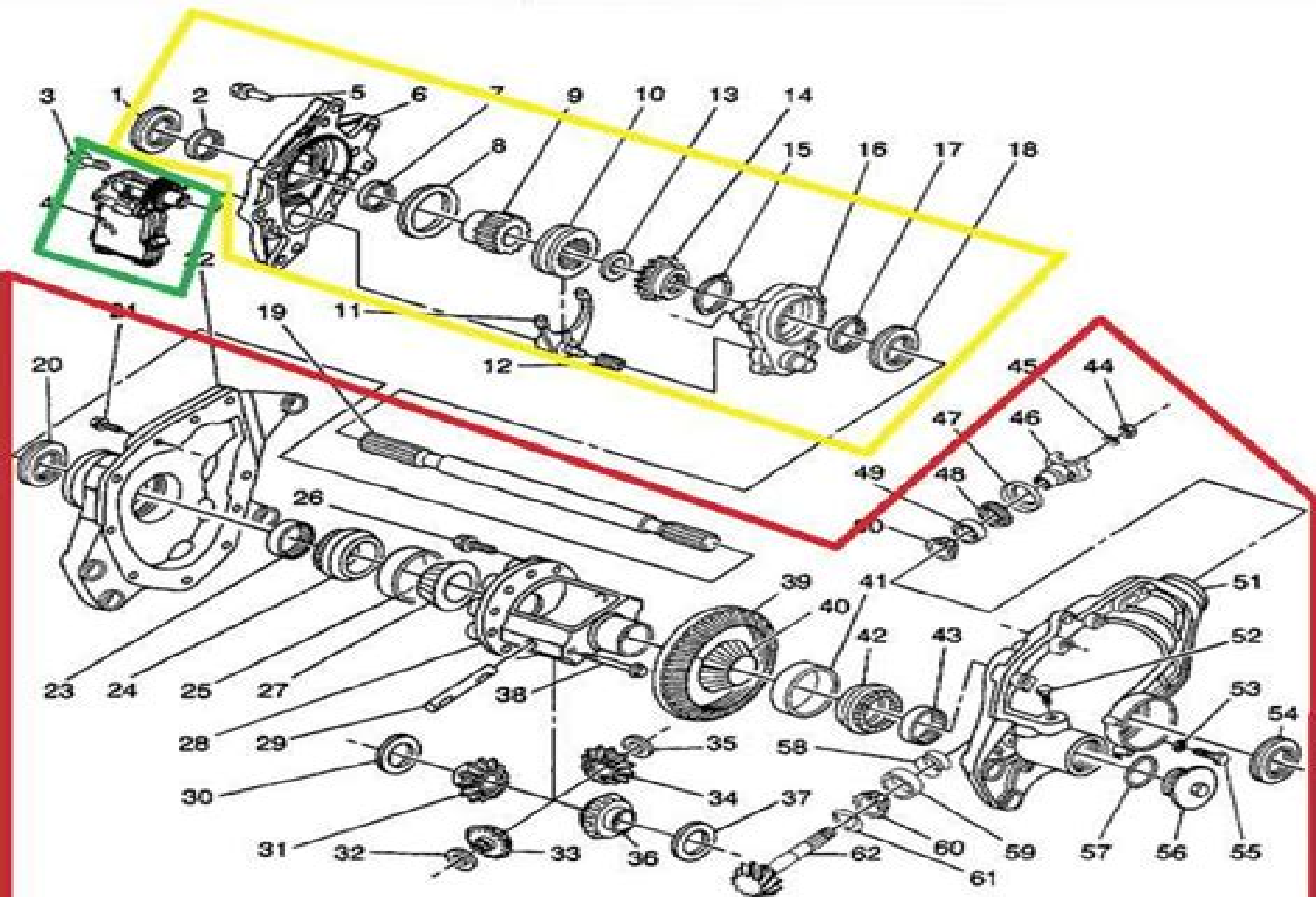
Fig. 1: Exploded View Front Drive Axle (7.25 in Axle) (S4WD)
