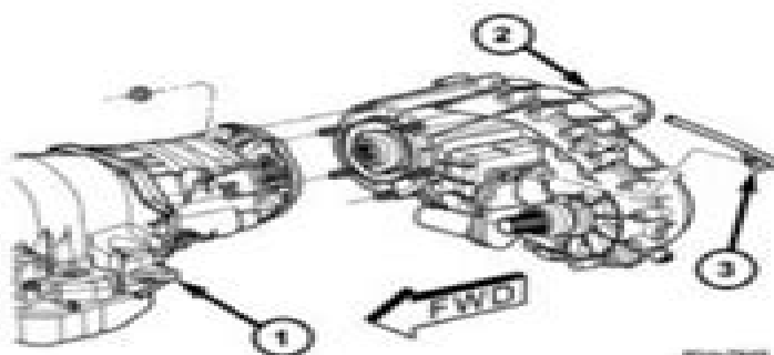
Fig. 2: Transmission, Transfer Case & Mode Sensor Connector Courtesy of CHRYSLER GROUP, LLC
