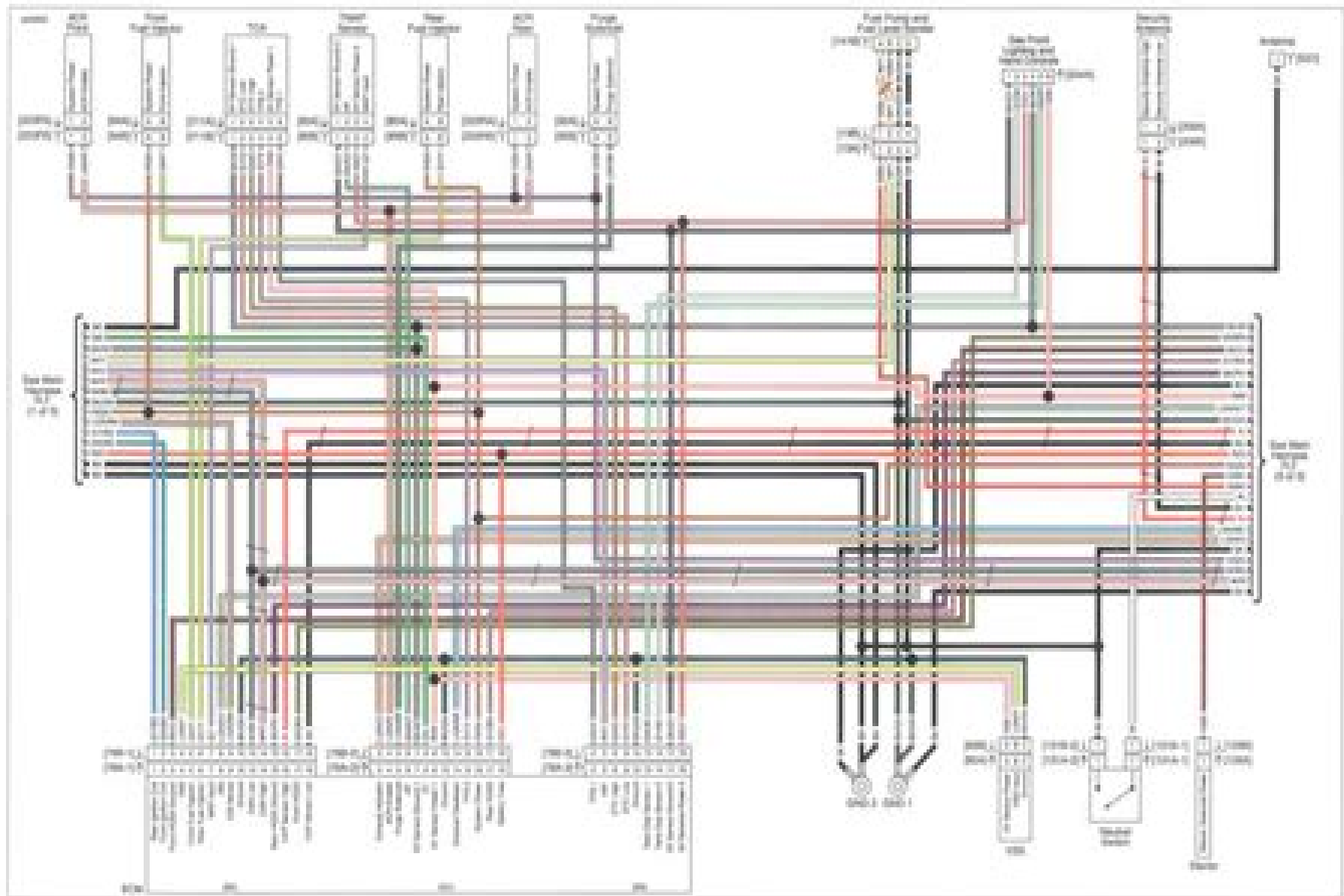
Figure 8-18. Main Harness PL7 (2 of 3) 2010 Testing
