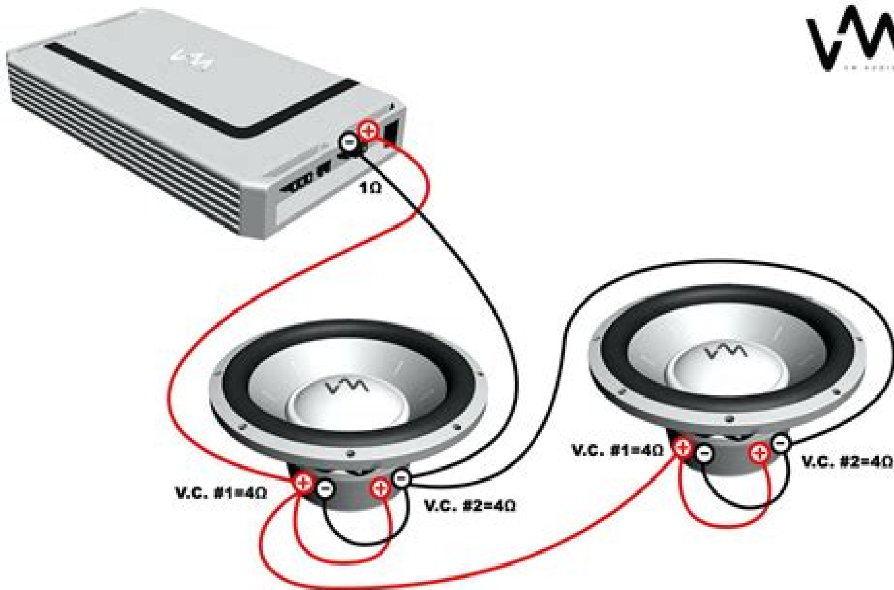
TWO 4Ω DVC SUBS, MONO AMP: 1Ω LOAD
