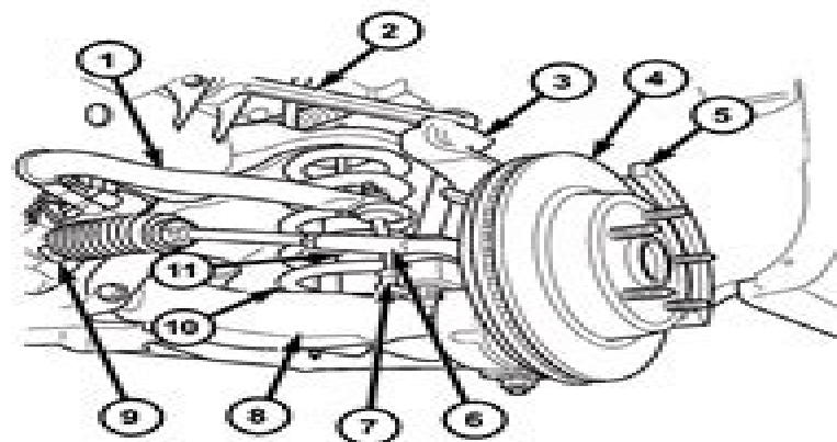
Fig. 1 FRONT SUSPENSION - 4X2
