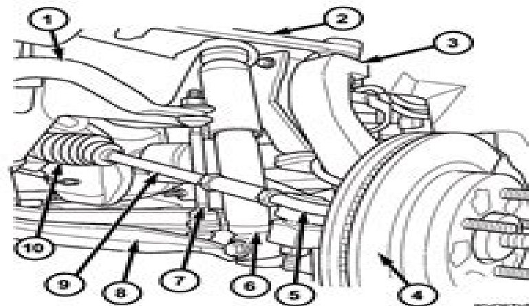
Fig. 2 FRONT SUSPENSION - 4X4 (LD ONLY)
