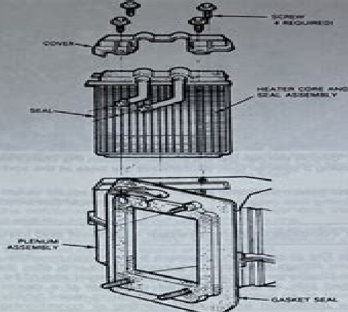
12.21 Remove the four screws and retaining cover, then lift the heater core from the plenum assembly
