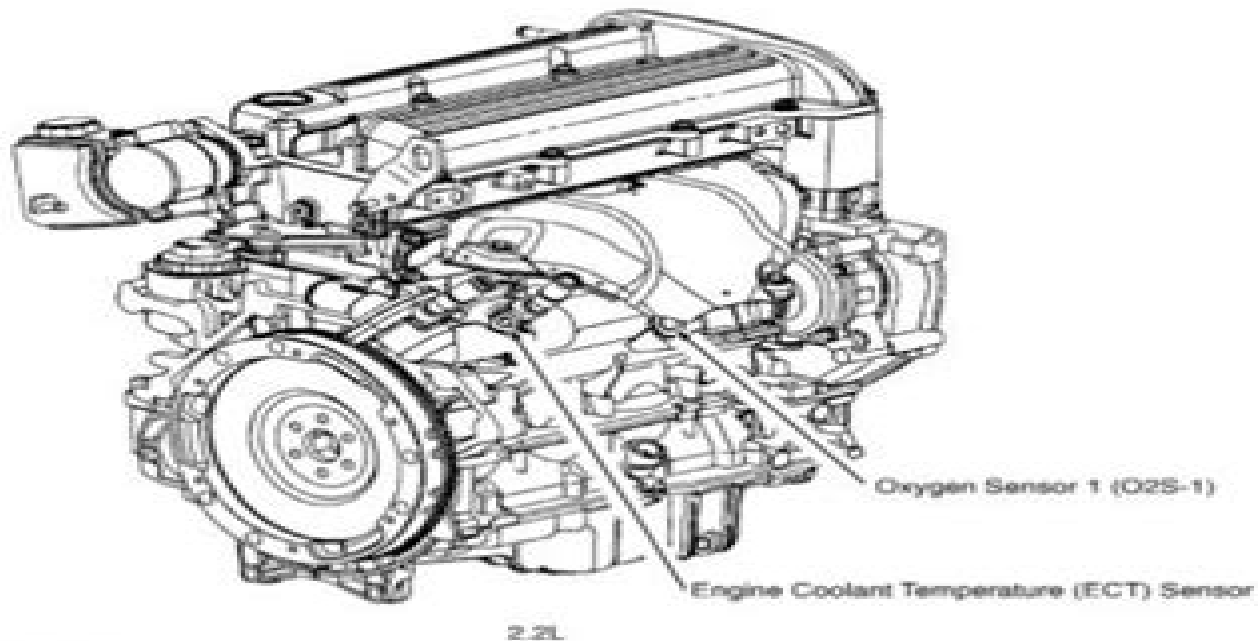
Fig. 2: Right Rear Of Engine (2.2L) Courtesy of GENERAL MOTORS CORP.
