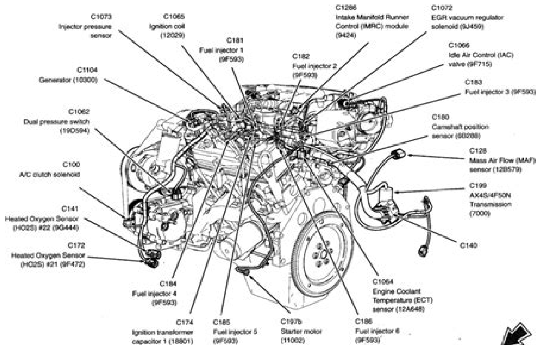
Fig. 1: Front Of Engine (2V)
