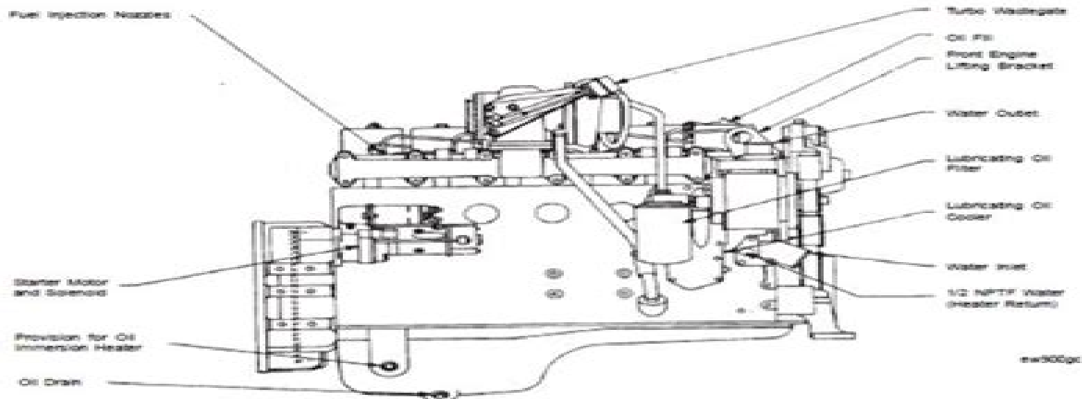
Turbocharger Side View
