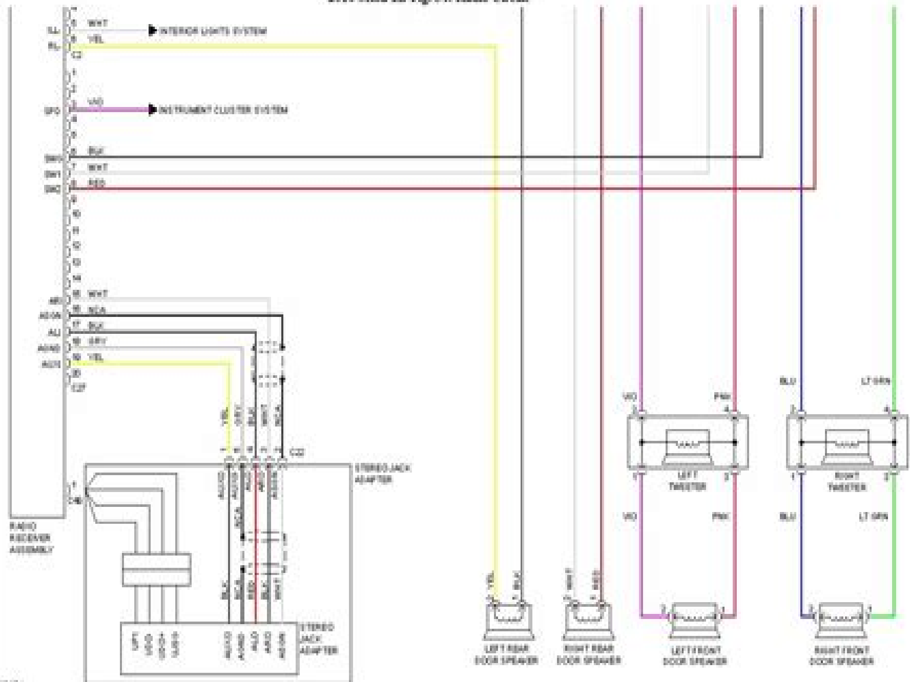
2010 Series nB-Fig. 34: Radio Circuit
