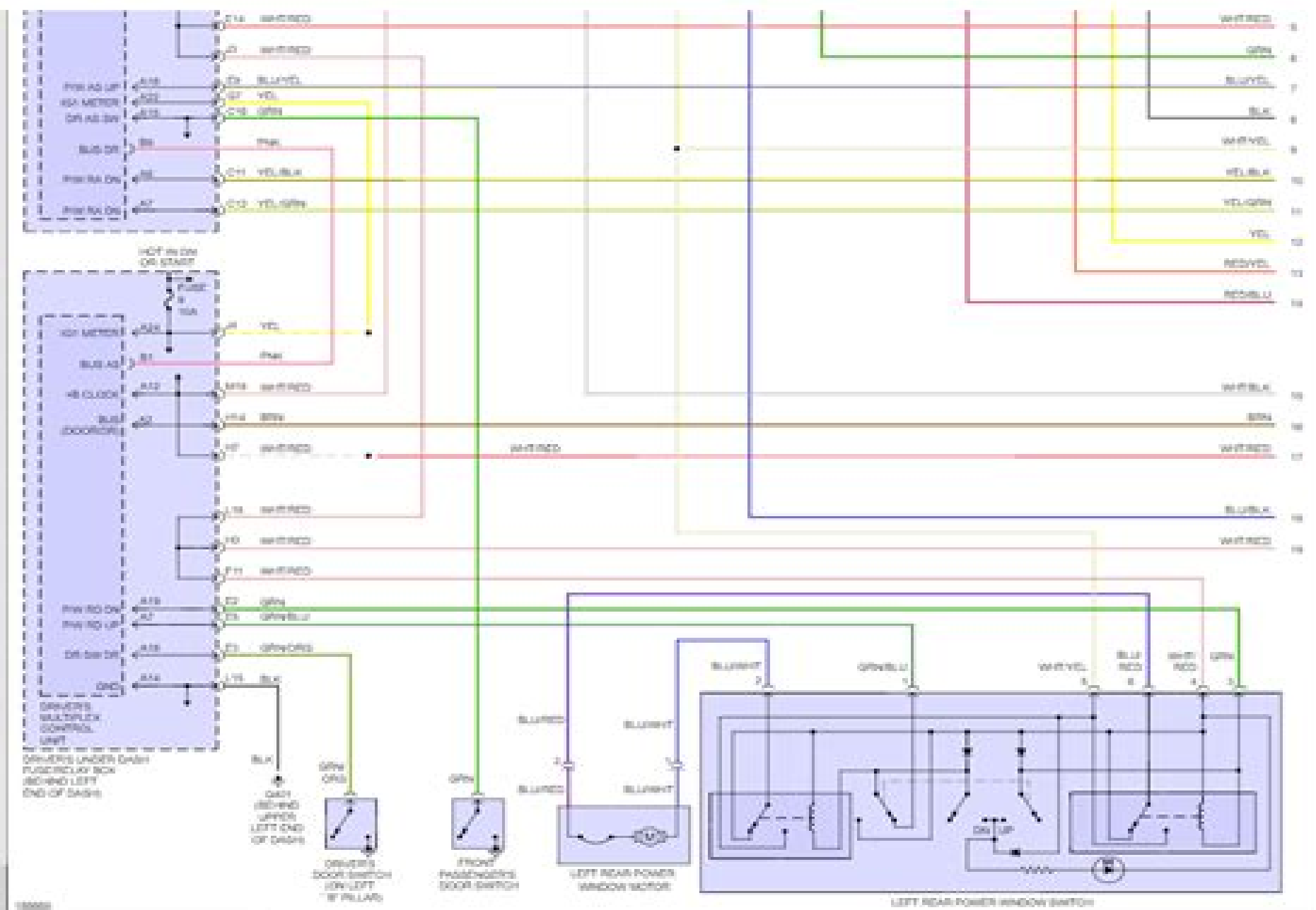
Fig 1: Power Windows Circuit (1 of 2)
