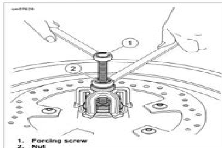
Figure 2-33. Removing Bearing
