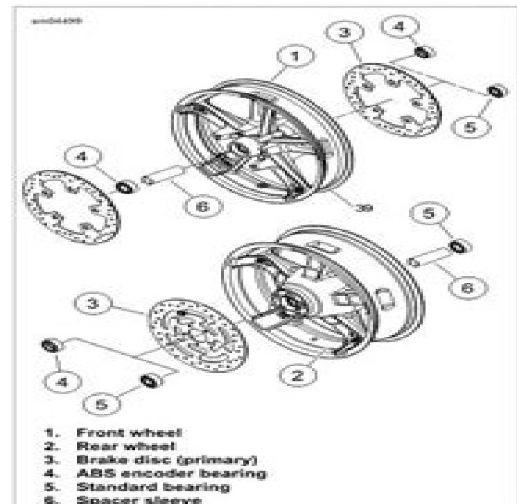
Figure 2-34. Wheel Bearing Assemblies
