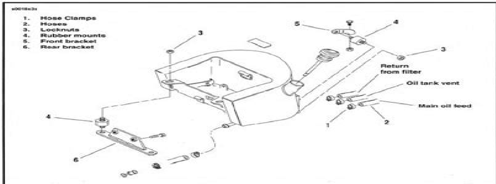
Figure 3-90. Softail Oil Tank
