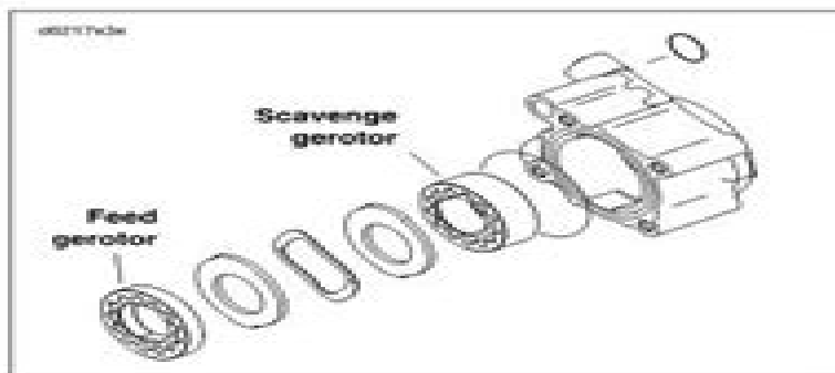
Figure 3-8. Oil Pump Gerotors
