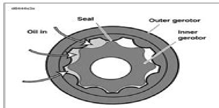
Figure 3-9. Inlet Side Oil Flow
