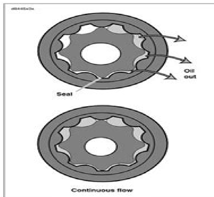
Figure 3-10. Outlet Side Oil Flow
