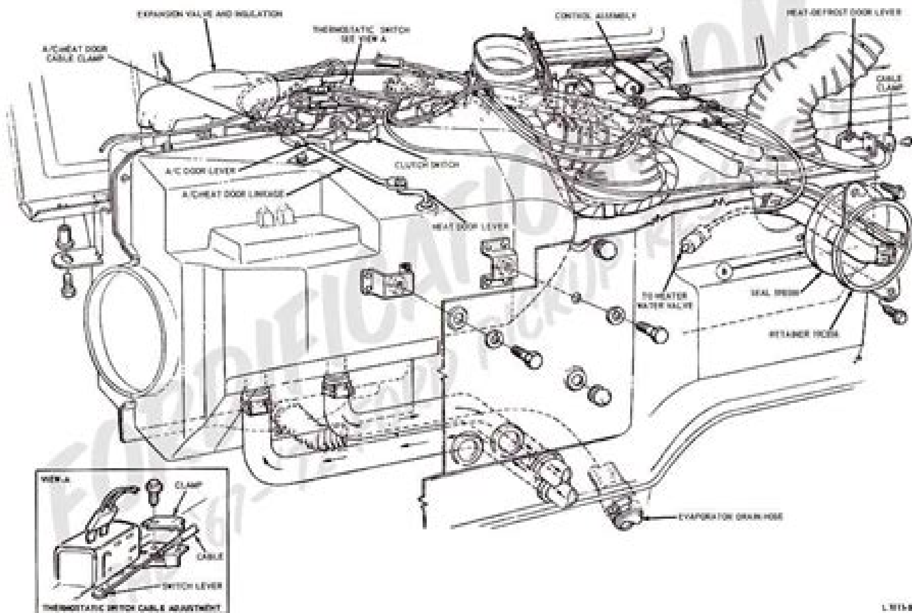
FIG. 3 Heater-Air Conditioner Installation—Light Truck
