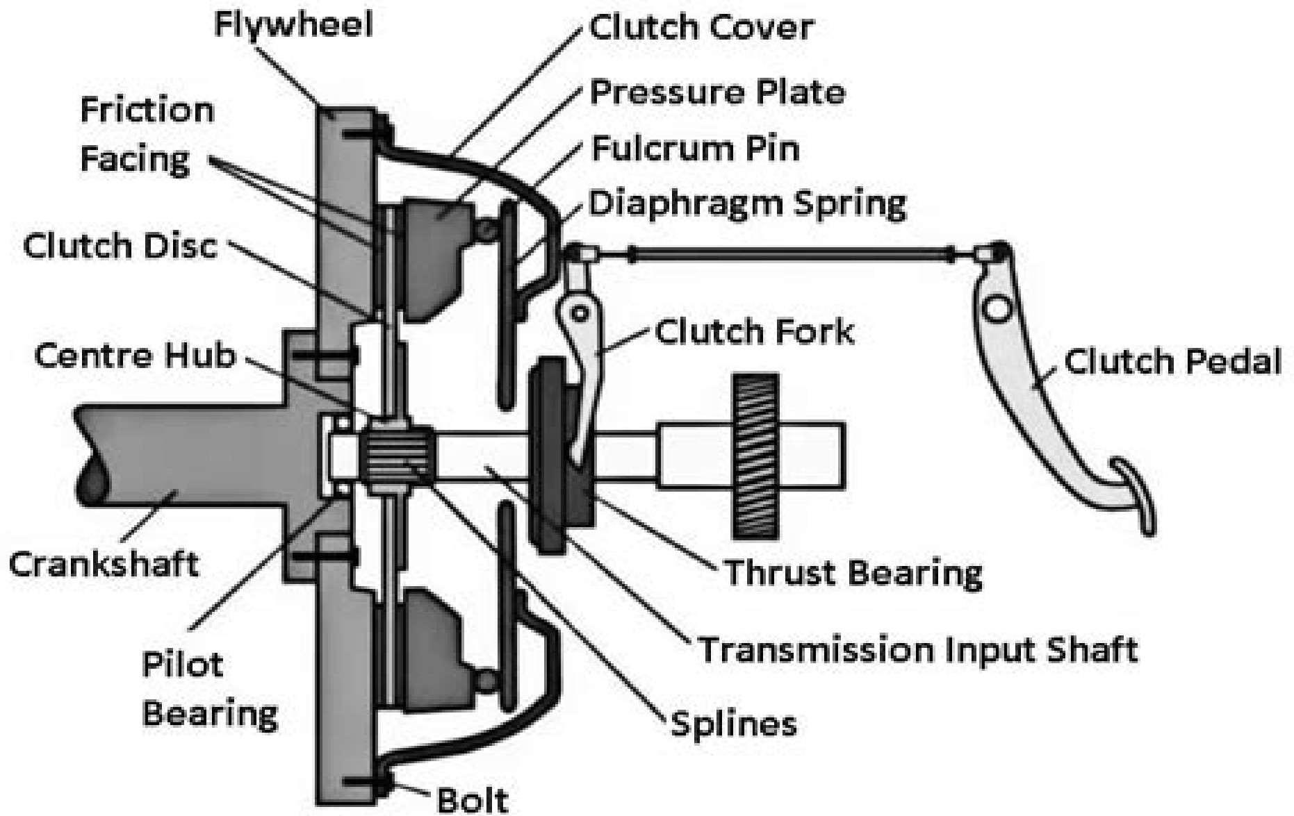
Parts of Single Plate Clutch
