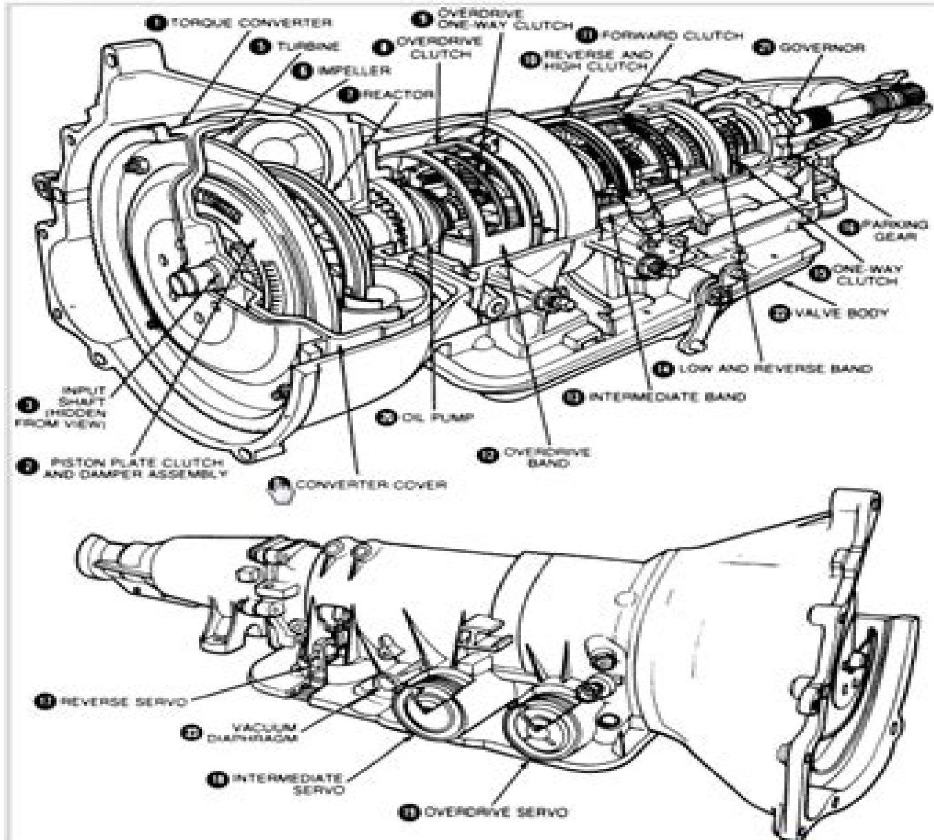
Cross-Sectional View Of A4LD Transmission
