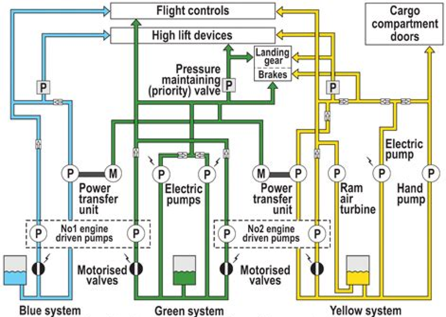
Typical twin engine hydraulic system layout
