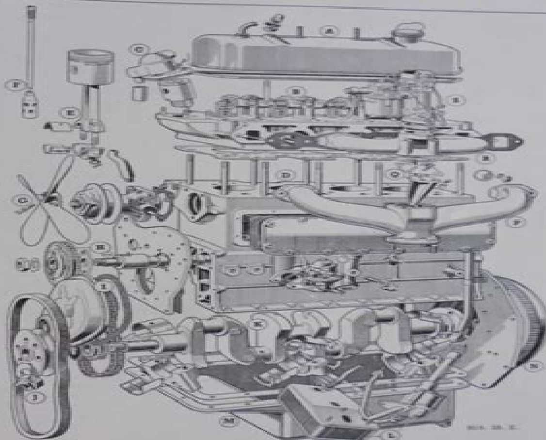
Fig. 1. An exploded view of the engine.
