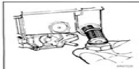
Fig. 36 In-carburetor fuel filter
