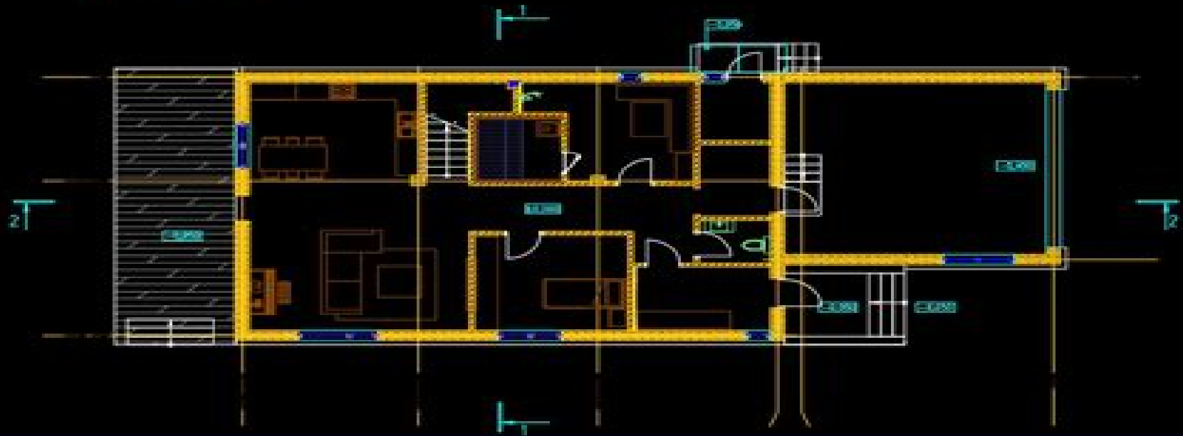
LEVEL GROUND
