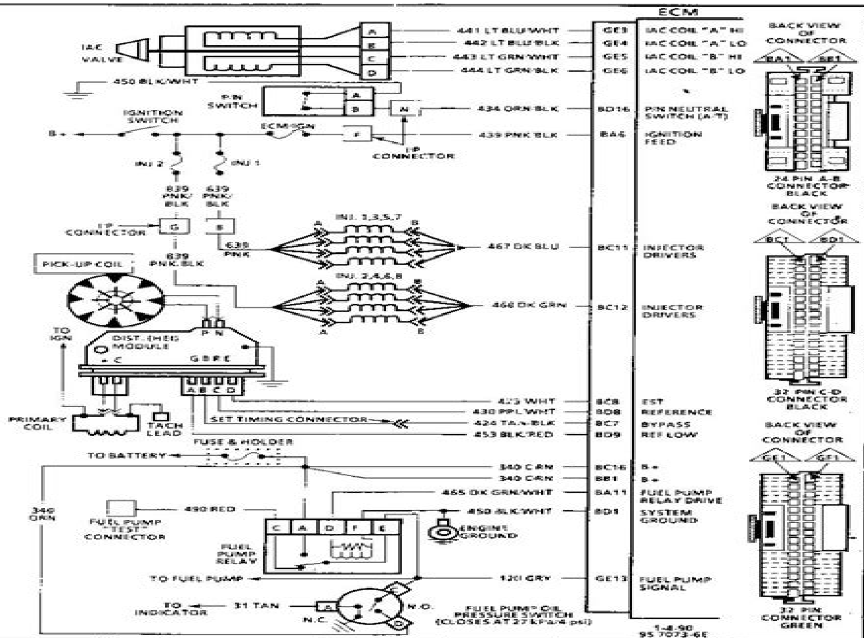
Figure A-3 - ECM Wiring Diagram 5.0L (VIN F) & 5.7L (VIN 8) "F" Carline (2 of 4)
