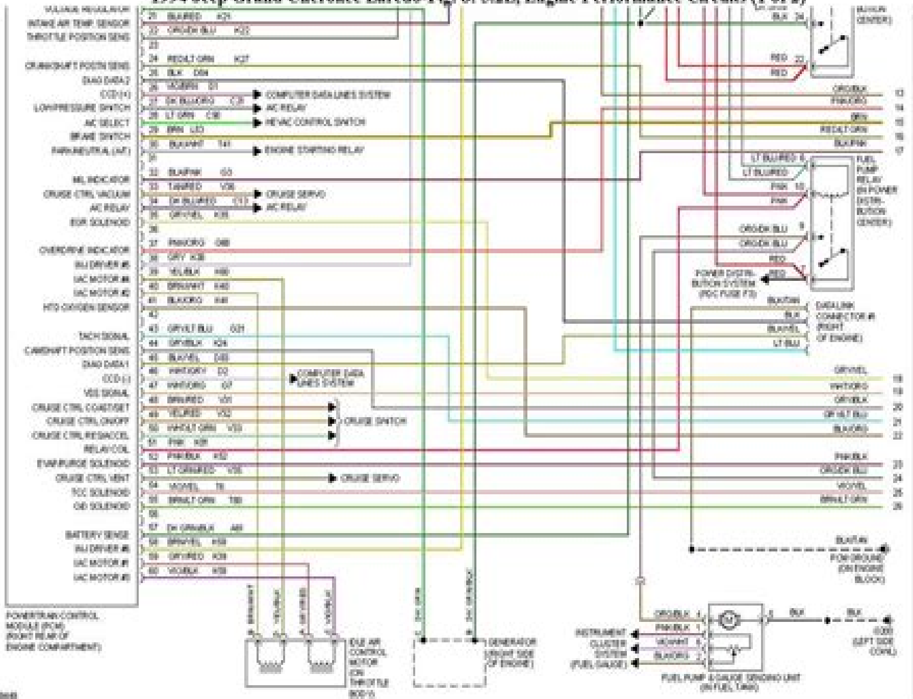
1994 Jeep Grand Cherokee Laredo-Fig. 8: 5.2L, Engine Performance Circuits (1 of 2)
