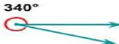
Reflex Angle
