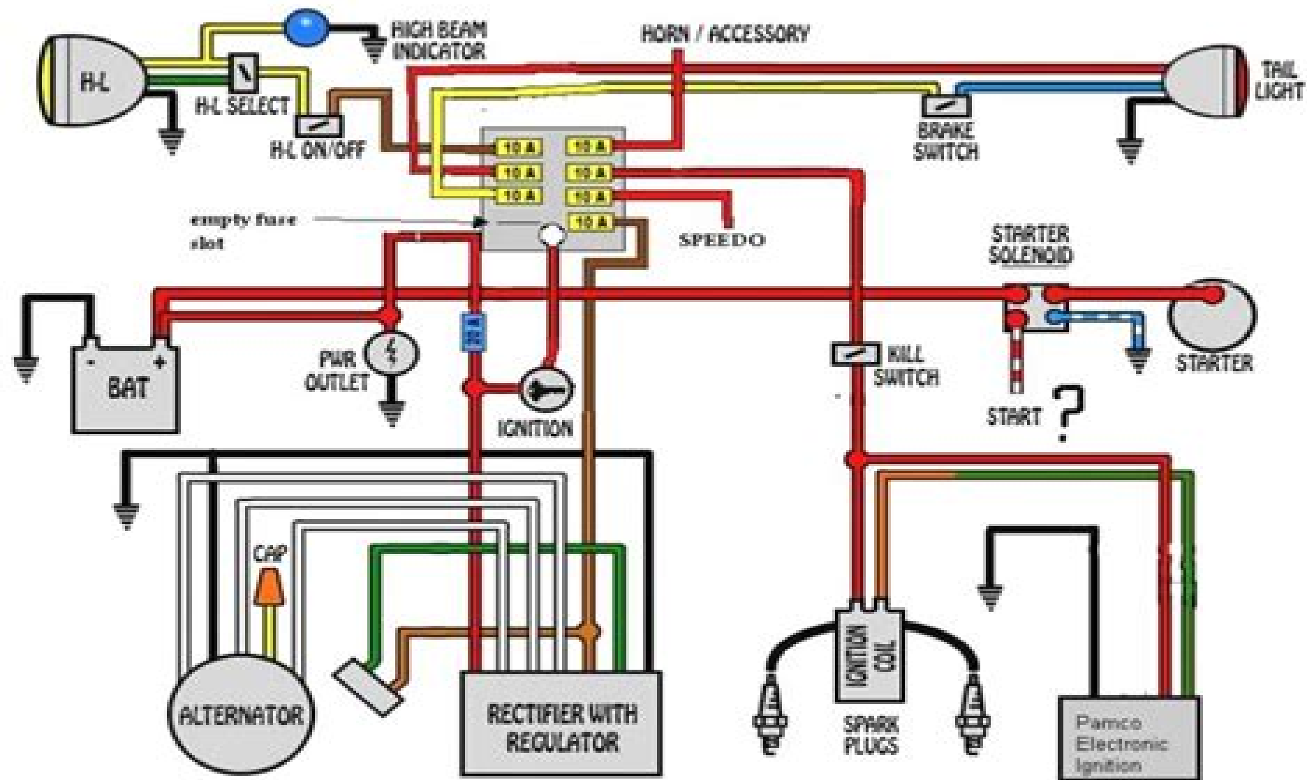
Motorcycle Electrical Wiring Diagram
