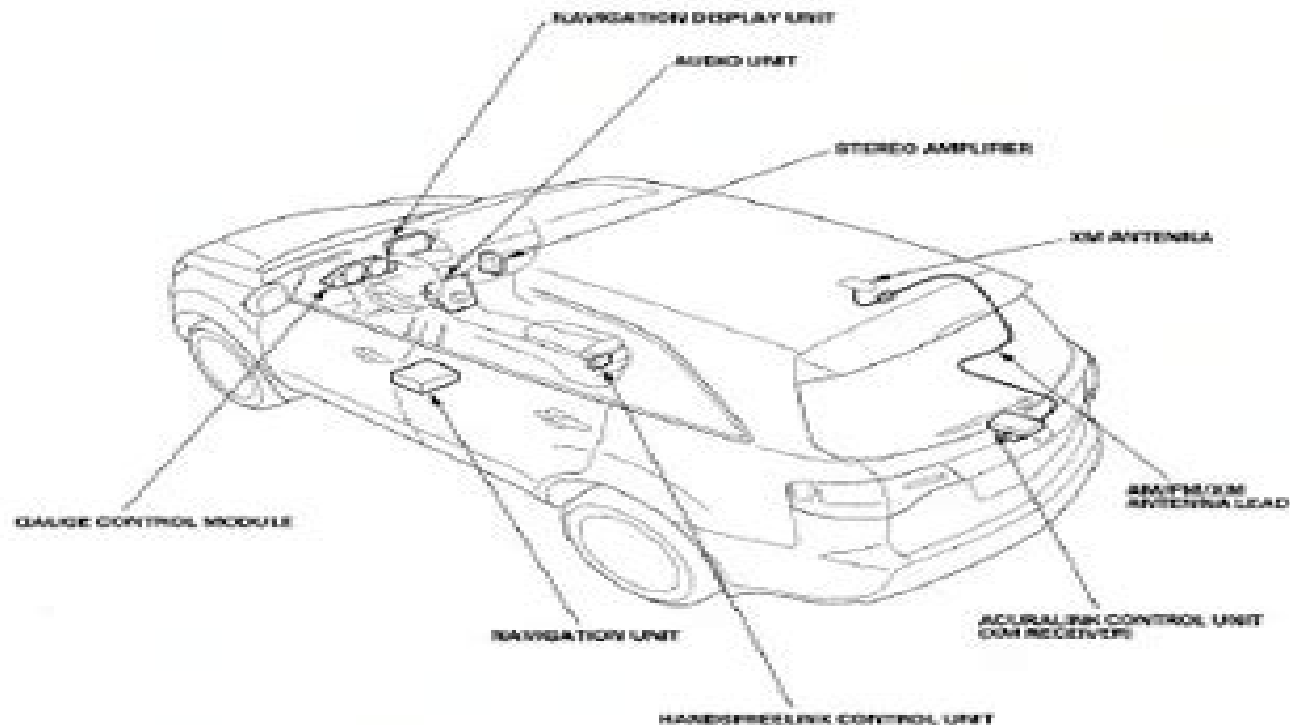
Fig. 1: Identifying AcuraLink Components; Courtesy of AMERICAN HONDA MOTOR CO., INC.
