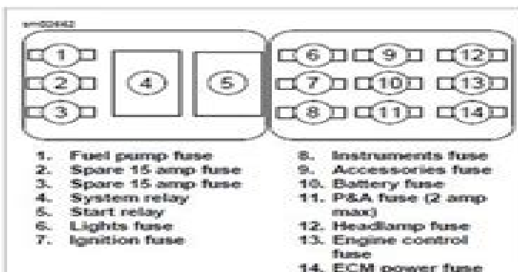
Figure 8-12. Fuse Block: Top View
