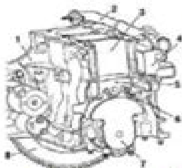
Fig. 1.19. Cooling of the piston: 1 - the engine block, 2 - pipe cooling system, 3 - cylinder walls, 4 - oil cooler, 5 - piston, 6 - oil spray atomizer, 7 - crankshaft
